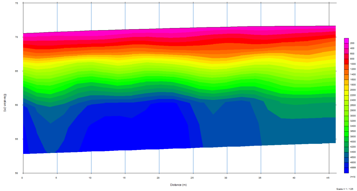
Fig B.1: Tomographic inversion for S1, plotted SW-NE.
