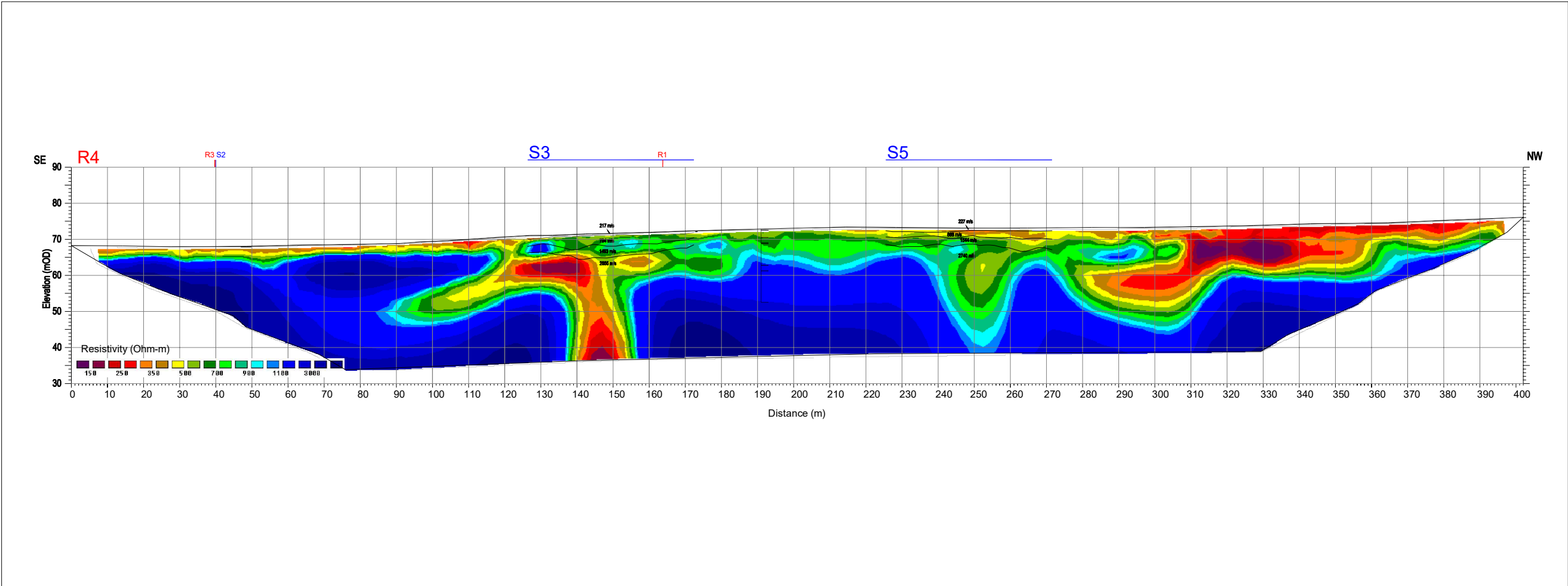
FIG.2.INTERPRETATION ERT R4 AND SEISMIC REFRACTION S3 & S5 SCALE 1:1250
