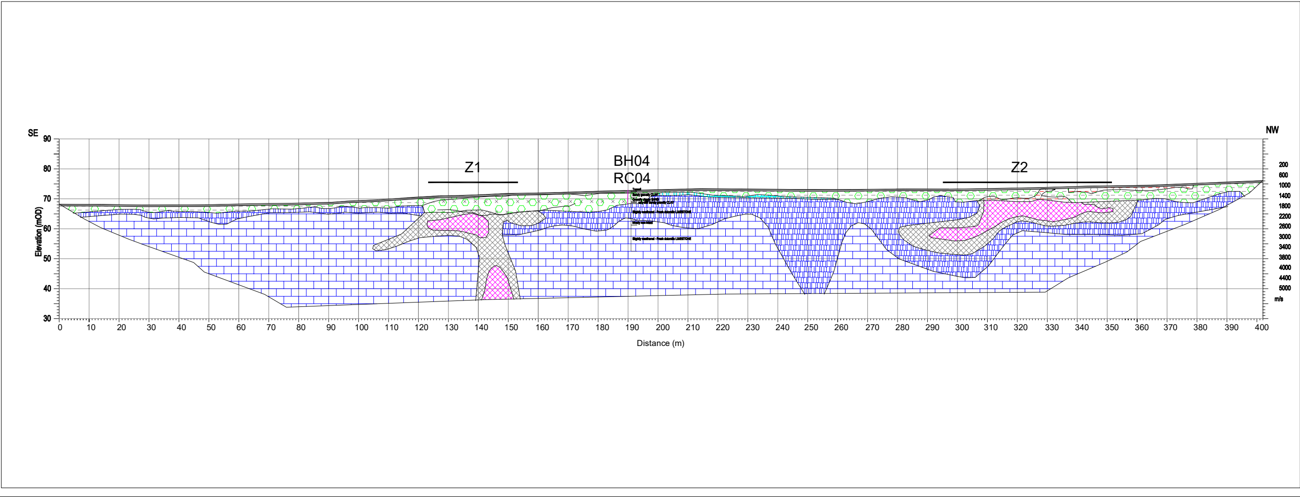
FIG.2.INTERPRETATION ERT R4 AND SEISMIC REFRACTION S3 & S5 SCALE 1:1250
