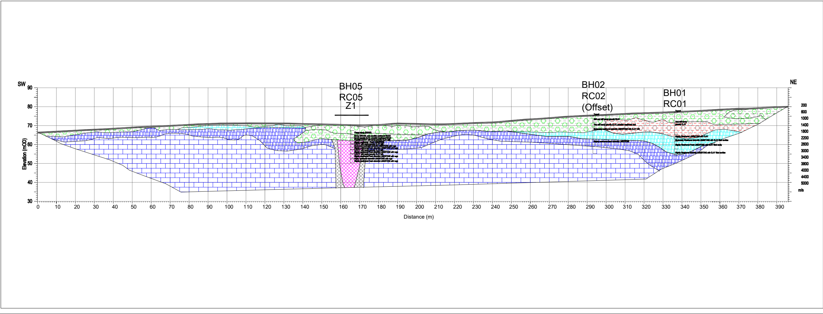
FIG.2.INTERPRETATION ERT R2 AND SEISMIC REFRACTION S1 & S6 SCALE 1:1250
