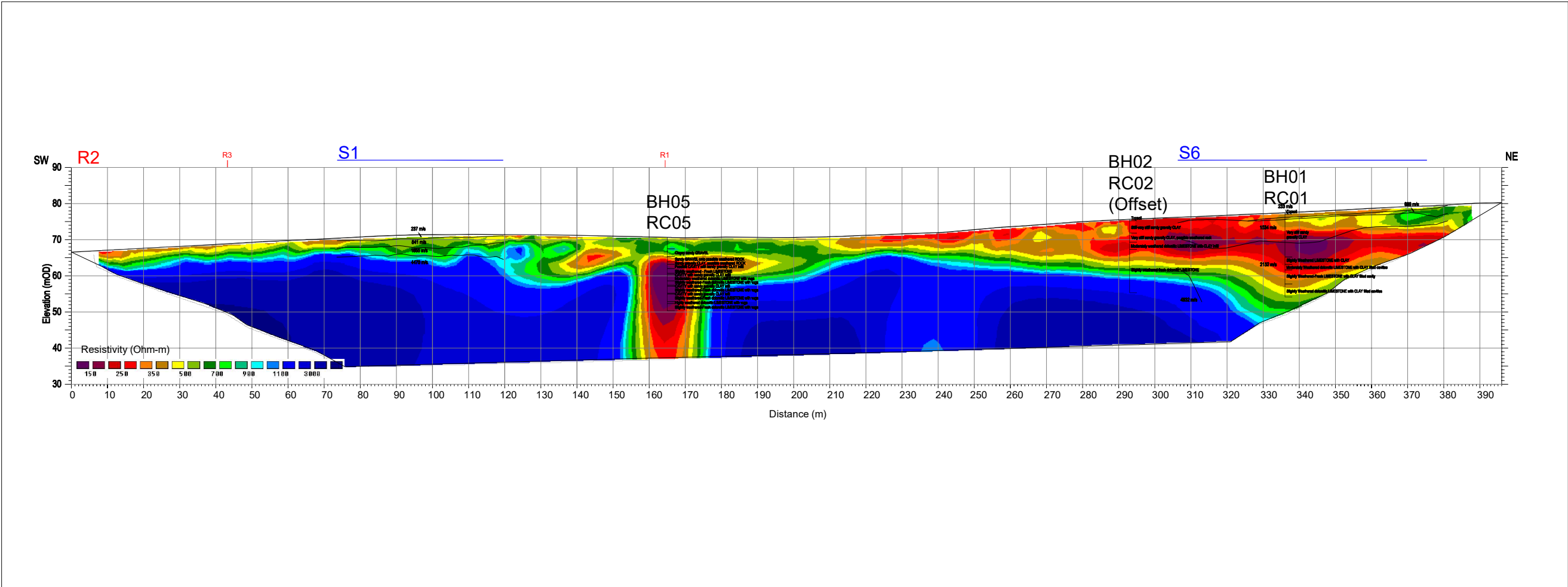
FIG.2.INTERPRETATION ERT R2 AND SEISMIC REFRACTION S1 & S6 SCALE 1:1250
